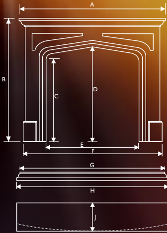
Dimensions are accurate to within +/- 6mm (1/4")
